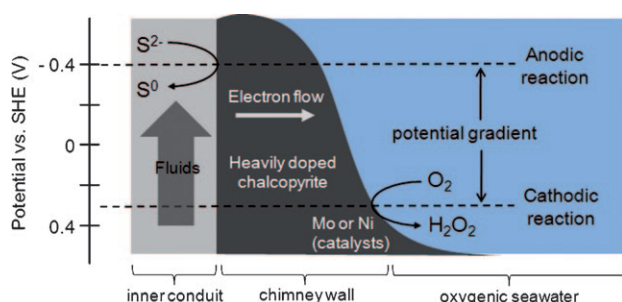
Figure 4. Schematic illustration of an energy diagram for the anodic and cathodic reactions occurring at the inner and outer surfaces, respectively, of the chimney. The potential gradient across the chimney serves as a driving force for electrical current generation.
